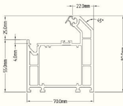
Slim 65mm PVC Frame*
