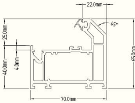
Standard 80mm PVC Frame*
